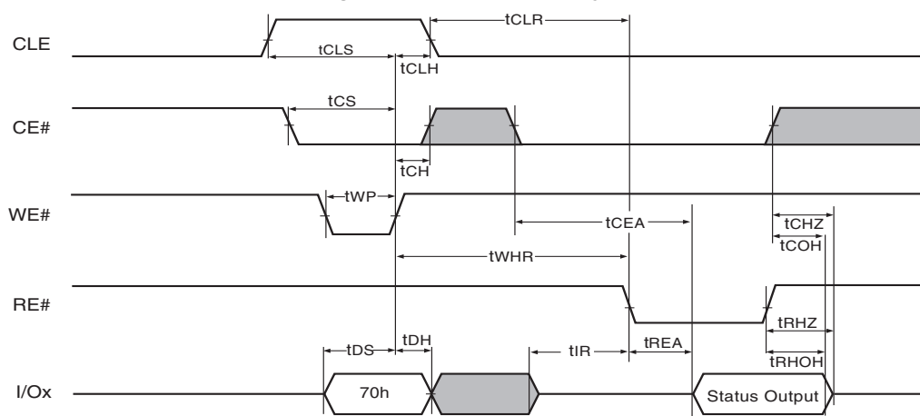
Figure 6.16 Status Read Cycle
