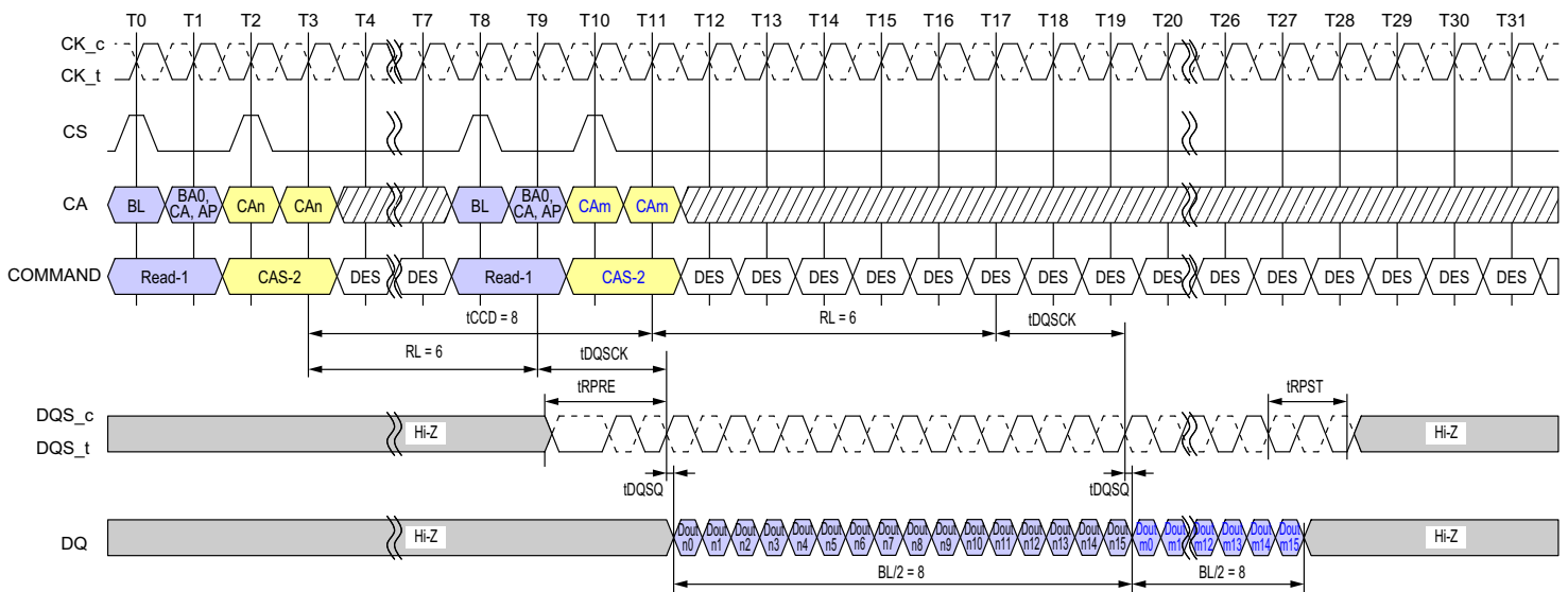
Figure 30 - Seamless Reads Operation: t_{CCD} = \text{Min} , Preamble = Toggle, 1.5nCK Postamble
