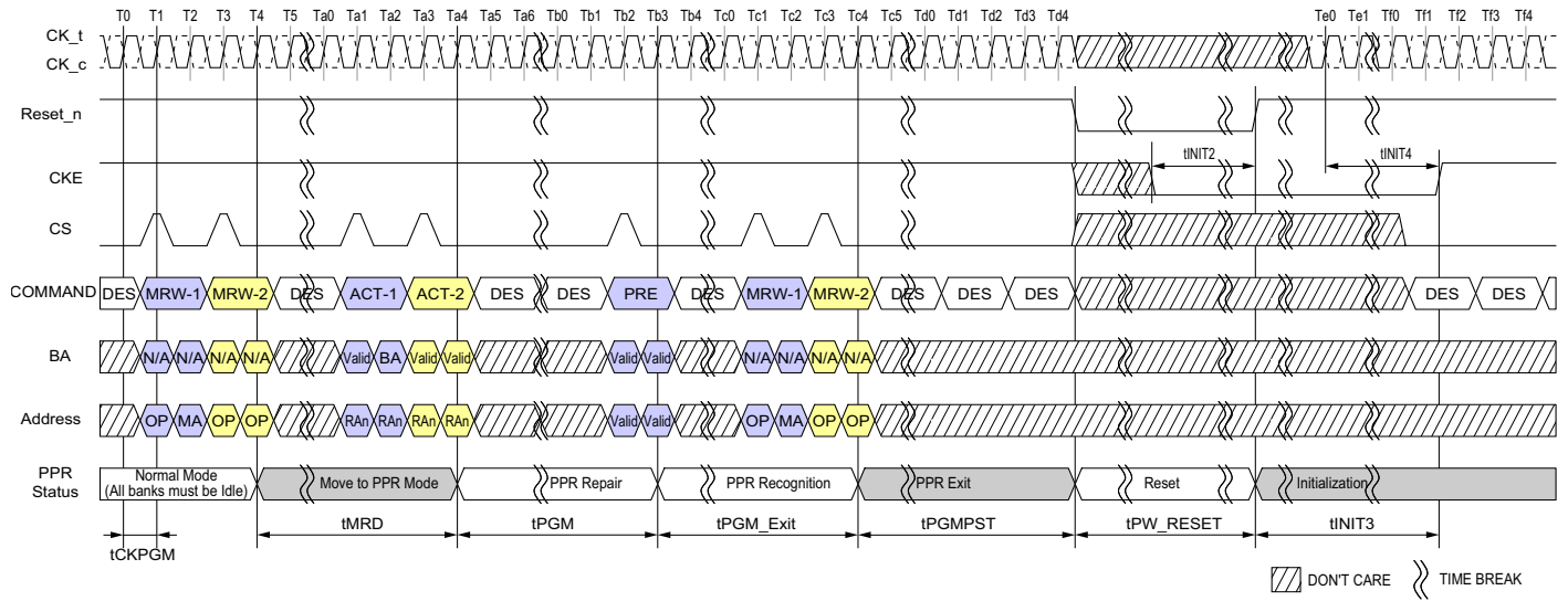
Figure 153 - PPR Timing
