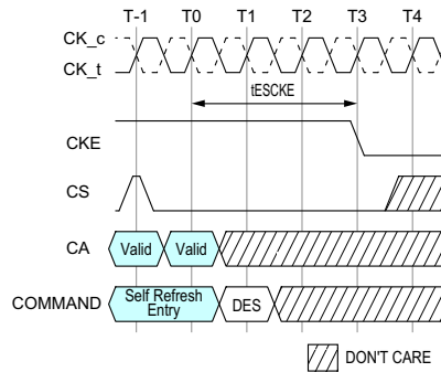
Figure 75 - tESCKE Timing
