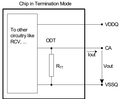
Figure 134 - CA On Die Termination
