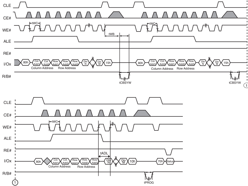
Figure 6.23 Cache Program
