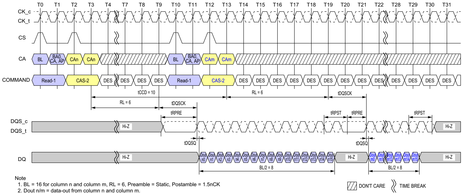
Figure 37 - Consecutive Reads Operation: tCCD = Min + 2, Preamble = Static, 1.5nCK Postamble
