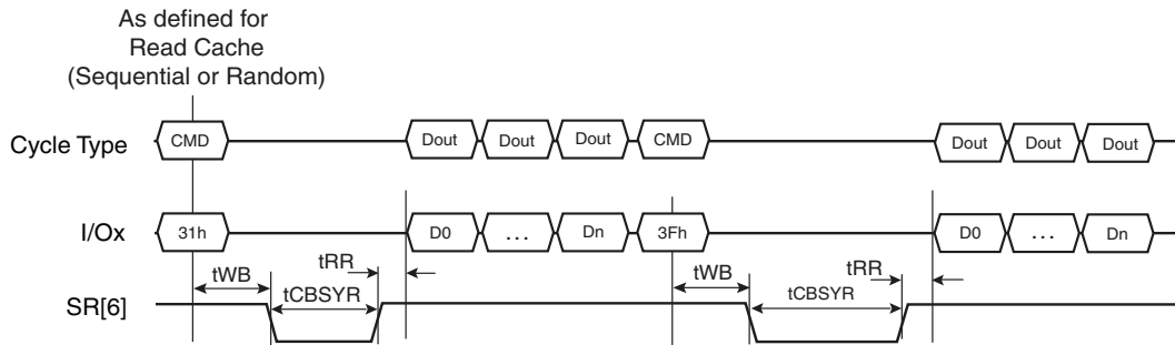
Figure 6.22 Read Cache Timing, End Of Cache Operation
