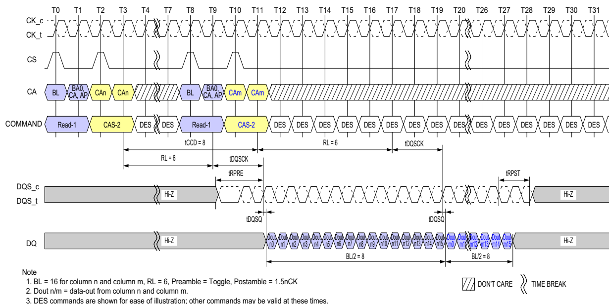
Figure 5 - Activate Command
