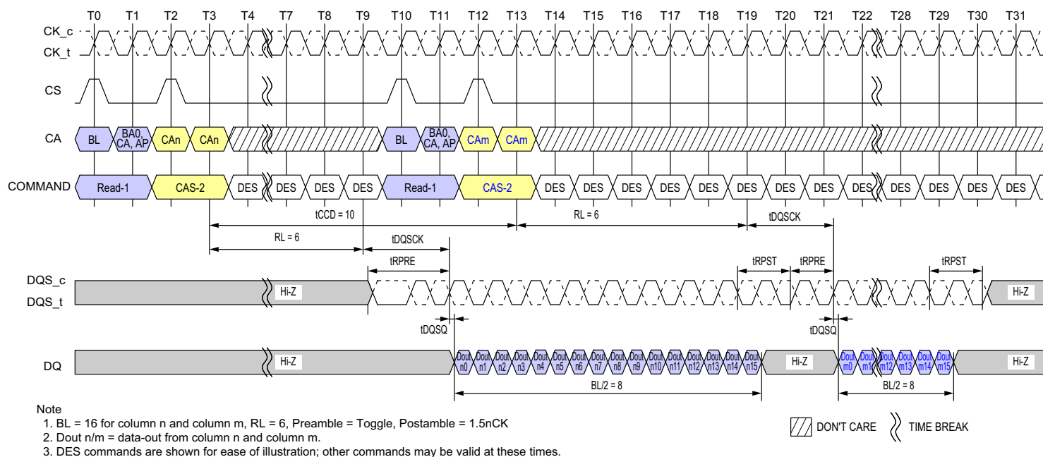
Figure 35 - Consecutive Reads Operation: tCCD = Min +2, Preamble = Toggle, 1.5nCK Postamble
