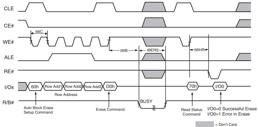
Figure 6.13 Block Erase Operation (Erase One Block)
