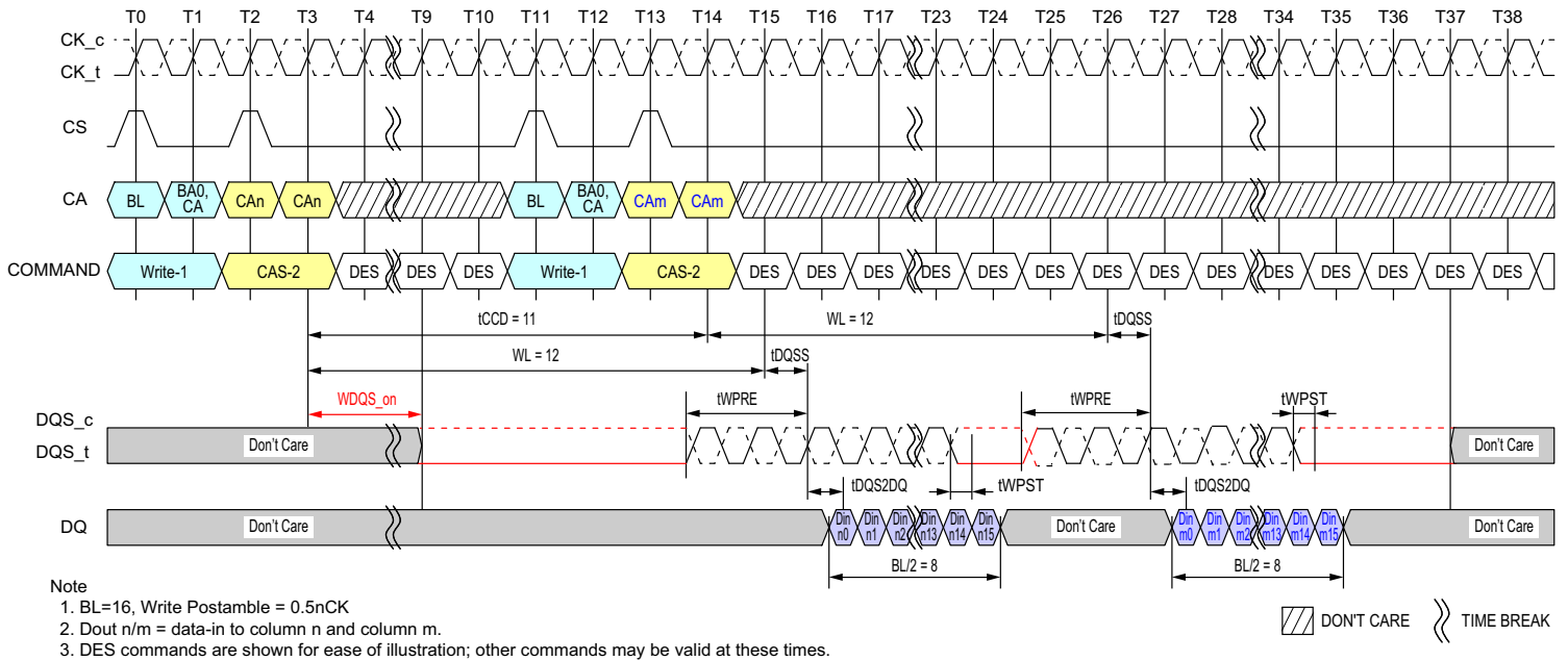
Figure 50 - Consecutive Writes Operation: t_{CCD} = \text{Min} + 3, 0.5nCK Postamble
